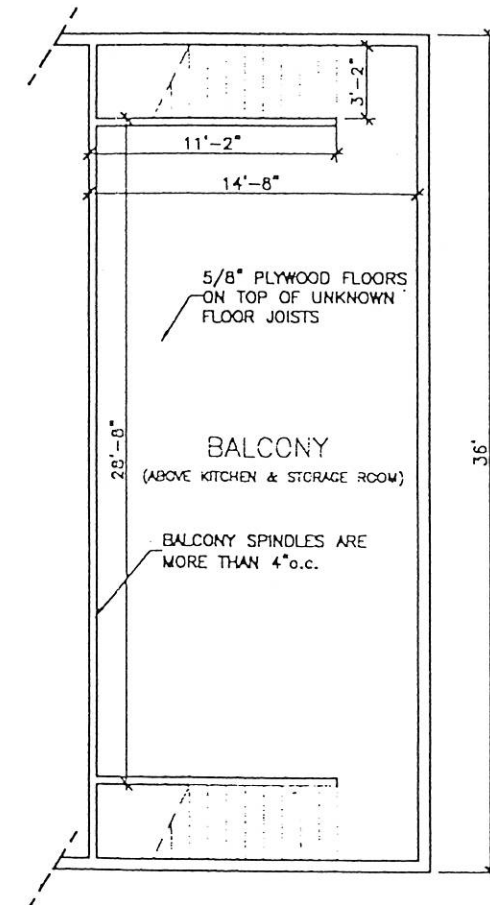
FLOOR PLAN—BALCONY SCALE: 1/8"=1'
